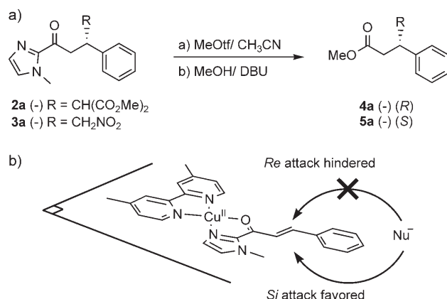
Scheme 2. a) Synthesis of 4a and 5a and b) schematic representation of the stereochemistry of the attack of the nucleophile in the DNA-based catalytic asymmetric Michael addition.
