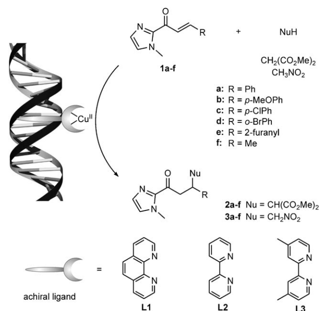
Scheme 1. Schematic representation of the asymmetric Michael addition reaction catalyzed by complexes formed between copper(II) ions and achiral ligands (L1–L3) in the presence of DNA.
